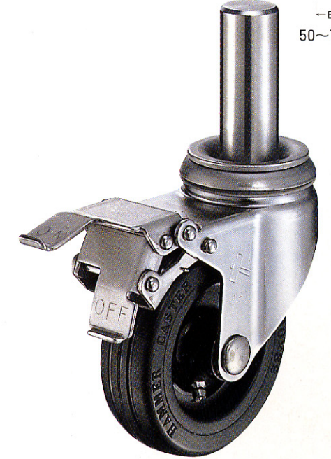
315SK-RU 100mm
